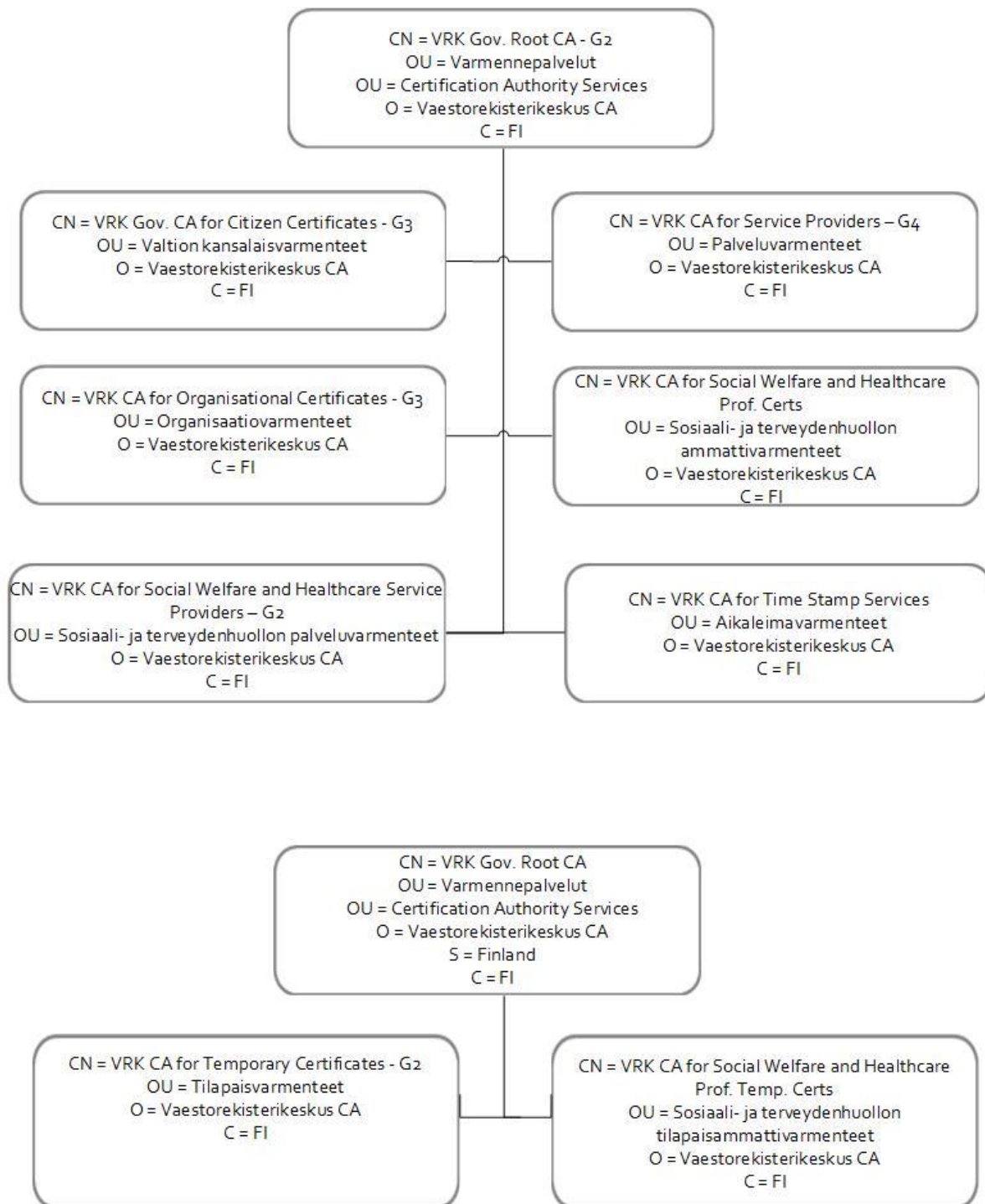
Figure 1: Certificate hierarchy
