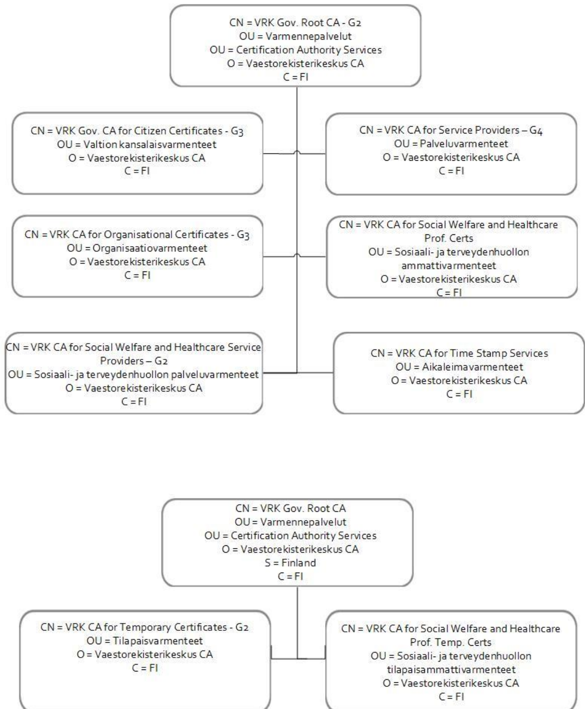
Figure 1: Certificate hierarchy
