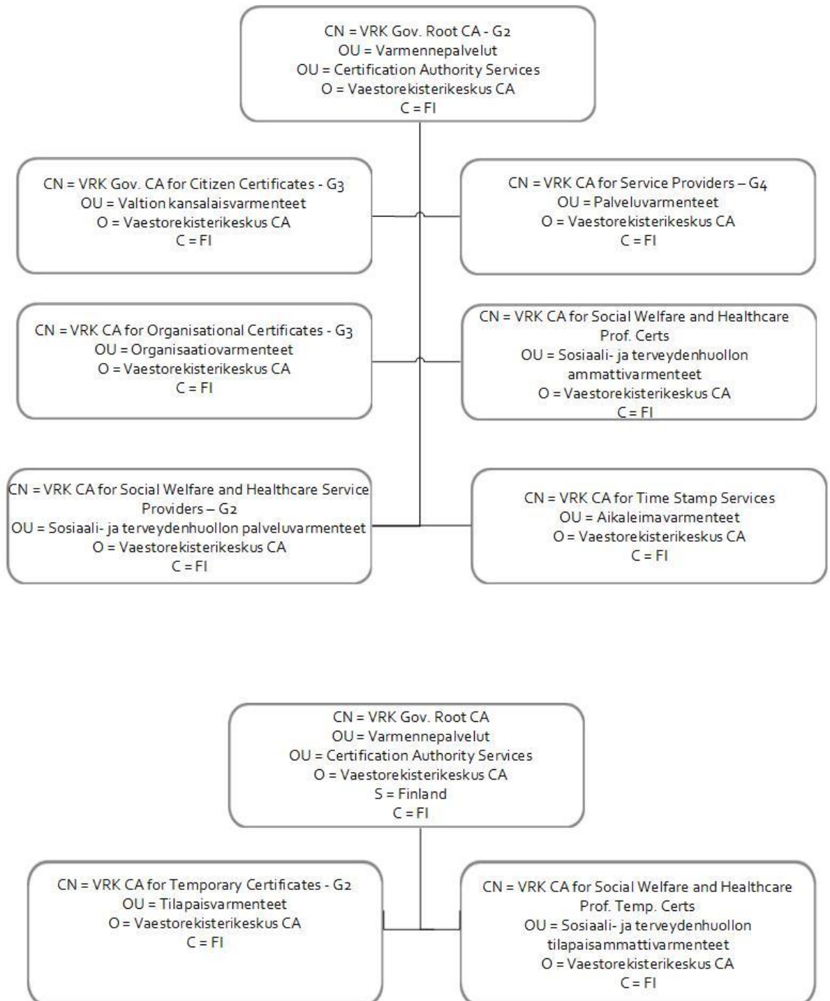
Figure 1: Certificate hierarchy
